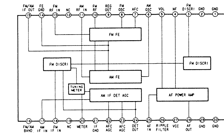
• IC Block Diagram IC1 CX1019S
