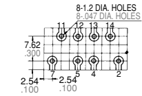
PC board pattern (Copper-side view)
