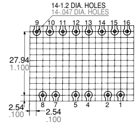
PC board pattern (Copper-side view)
